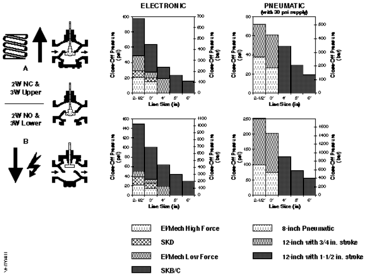
Figure 3. Close-off Pressures.
